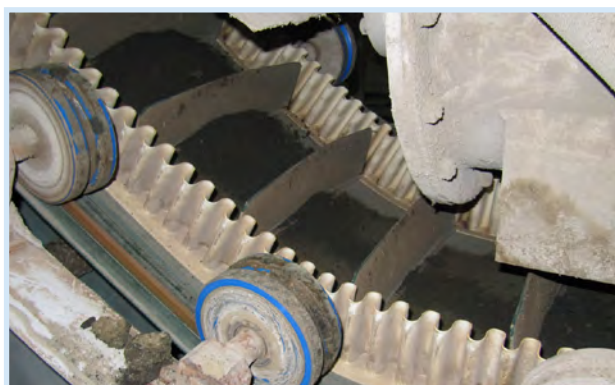
FRG-3 with thermo welded sidewalls and flights: CHEMICAL POWDER (RECYCLED SEWAGE)
